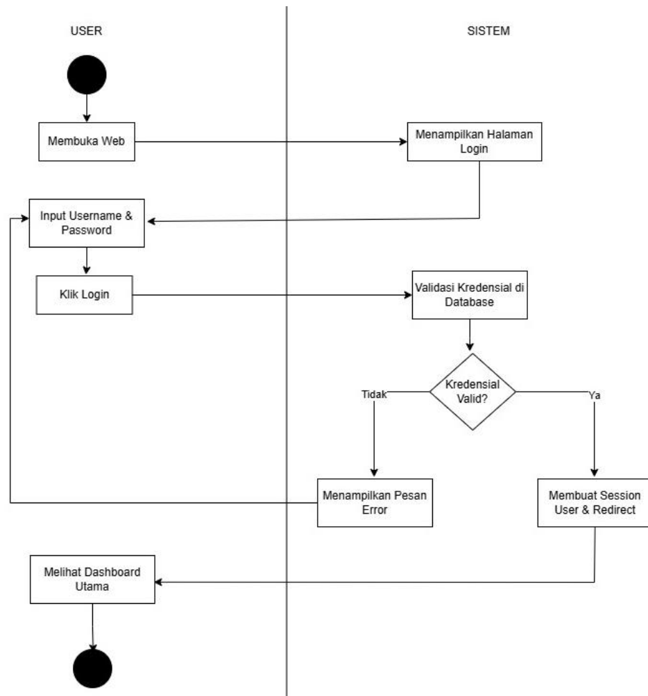
Gambar IV. 4 Activity Diagram Login
