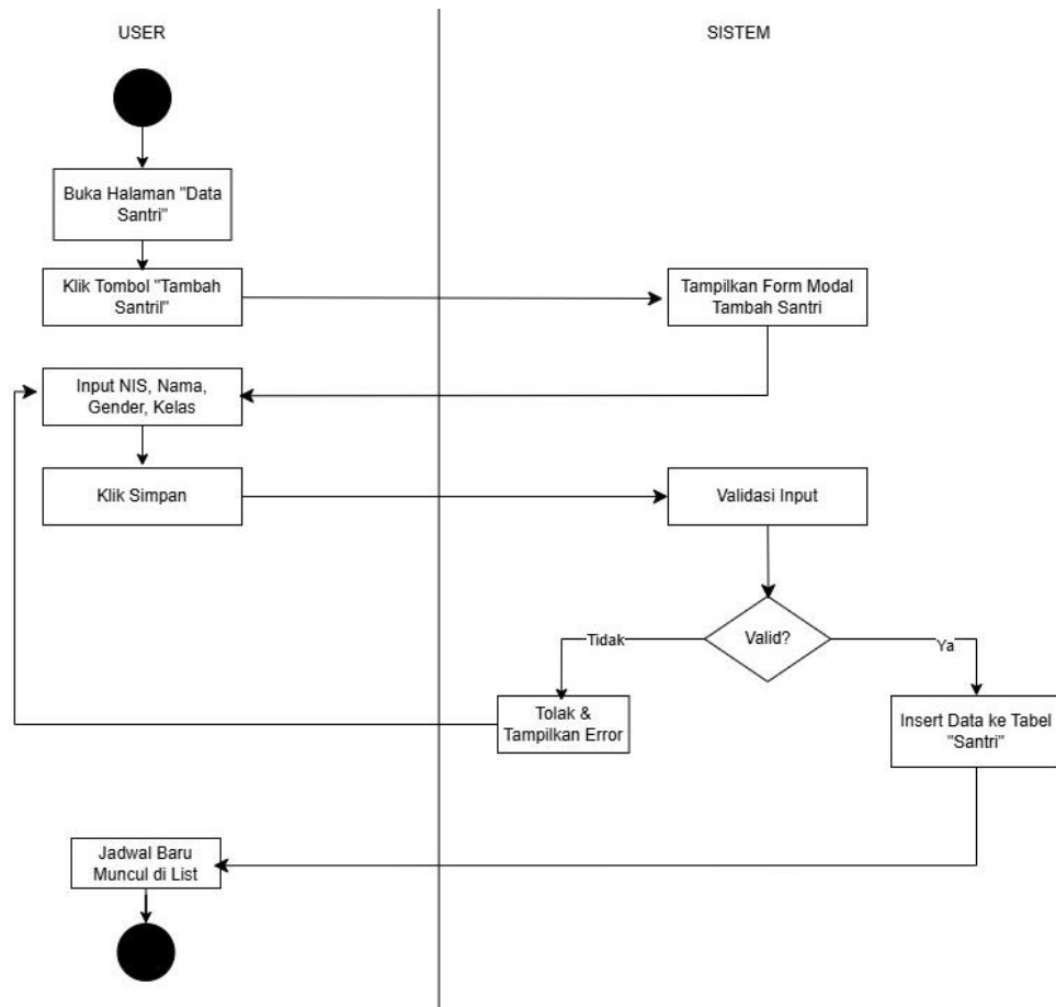
Gambar IV. 5 Activity Diagram Tambah Data Santri
