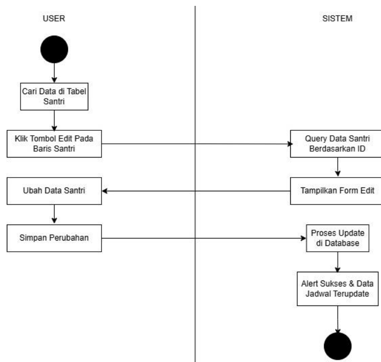
Gambar IV. 6 Activity Diagram Edit Data Santri
